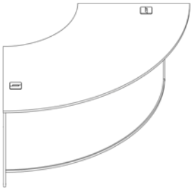
90° Outer Curved Starter VRCCS90*-** 2121(w) x 900(d) x 760(h)mm
