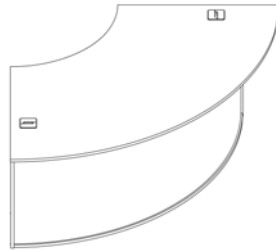
90° Outer Curved Mid VRCCM90*-** 2121(w) x 900(d) x 760(h)mm
