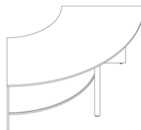
90° Outer Curved DDA VRCCD90*-** 2121(w) x 900(d) x 760(h)mm
