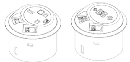
VTP1 Power Unit. 1x power, 1x USB, 1x data 3m Mains power lead 3m CAT5e UTP flyleads
